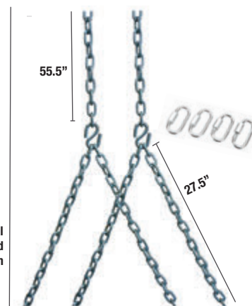
P0S0-CHN Heavy Duty Stainless Steel "Y" shape chain kit Weight: 7 lbs
