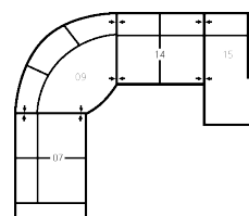
CONFIGURATION C4 140 x 114" 356 x 290cm
