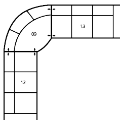
CONFIGURATION CA 139 x 139" 353 x 353cm
