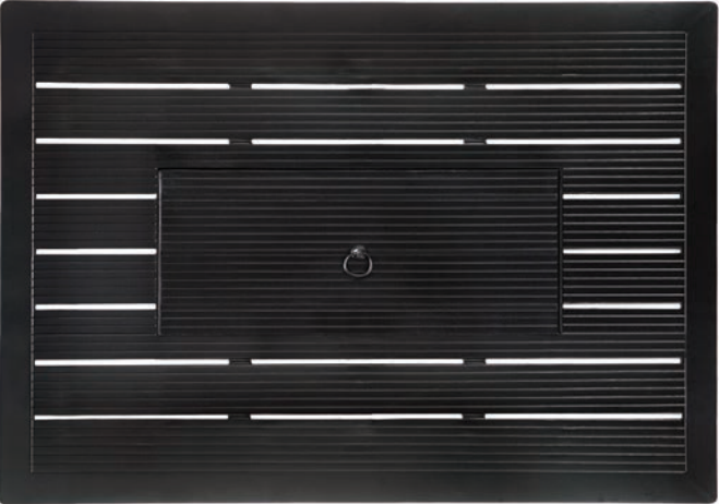
53" ROUND GAS FIRE PIT TOP | 1019GT53 W: 53" D: 53" H: 1.5" 40" X 56" RECTANGULAR GAS FIRE PIT TOP | 1019GTC7 W: 56" D: 40" H: 1.5" (shown at left)
