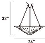
E20346-49 3-Light Pendant Finish: Satin Nickel Glass: Italian Ice 3 x 75W MB Lamps 3,450 Lumens 35" / 145" OAH
