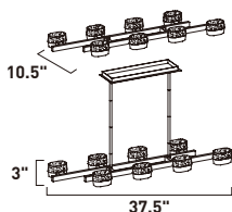
Frame diagram and overall measurements
