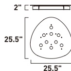
E20782-SF 9-Light Flush Mount Finish: Silver Foil 9 x 5W LED (Lamps Included) 2,900 Lumens
