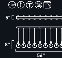
E23119-18 9-Light Pendant Finish: Polished Chrome Glass: Clear 9 x 20W G4 (Lamps Included) 2,880 Lumens 18" / 138" OAH
