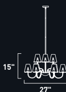
E20293-10 9-Light Chandelier Finish: Polished Chrome Glass: Clear 9 x 40W G9 (Lamps Included) 4,500 Lumens 21" / 46" OAH
