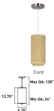
E95030-101OI E95030-101SN 1 x 75W MB Lamp • Includes tempered glass diffuser
