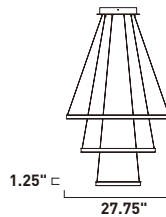
E22407-BZ 3-Tier LED Pendant Finish: Bronze Glass: Acrylic 100W LED (Integrated) 7,000 Lumens 20.5" / 47.25" OAH
