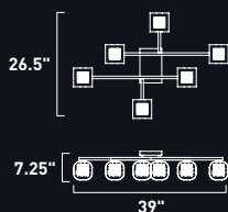
E22836-18SVPC E22836-18PCPC 6-Light Flush Mount Finish: Polished Chrome Glass: Clear 6 x 40W G9 (Lamps Included) 3,000 Lumens
