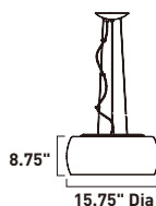
E21205-10PC 5-Light Pendant Finish: Polished Chrome Glass: Mirror Chrome 5 x 40W G9 (Lamps Included) 2,500 Lumens 18" / 120" OAH
