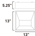
E21362-61BK LED Flush Mount/Wall Mount Finish: Black 20W LED (Lamps Included) 1,200 Lumens
