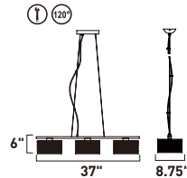
E21304-10PC E21304-10PC/BUL 3-Light Pendant Finish: Polished Chrome Metal Shade: Steel Web 3 x 75W G9 (Lamps Included) 3,900 Lumens 18" / 120" OAH
