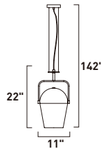
E20833-SA 1-Light Pendant Finish: Satin Aluminum 1 x 15W COB LED (Lamp Included) 1,650 Lumens 22" / 142" OAH
