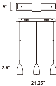
E22243-PC 3-Light LED Pendant Finish: Polished Chrome Shade: Polished Chrome 3 x 7.2W LED (Integrated) 468 Lumens 10" / 120" OAH (I) (D) (LED)
