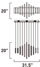
E22716-PC LED Pendant Finish: Polished Chrome Glass: Acrylic 65.2W LED (Integrated) 4,561 Lumens 23" / 143" OAH
