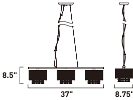
E23138-10PC 3-Light Pendant Finish: Polished Chrome Shade: Aluminum 3 x 60W G9 (Lamps Included) 2,400 Lumens 13" / 126" OAH
