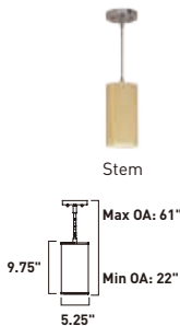
E95022-101OI E95022-101SN 1 x 60W MB Lamp • Includes tempered glass diffuser
