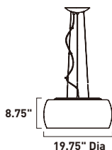
E21206-10PC 6-Light Pendant Finish: Polished Chrome Glass: Mirror Chrome 6 x 40W G9 (Lamps Included) 3,000 Lumens 18" / 120" OAH
