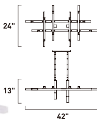
Frame diagram and overall measurements
