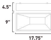
E21366-61BK LED Flush Mount/Wall Mount Finish: Black 20W LED (Lamps Included) 1,200 Lumens
