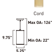
E95120-101OI E95120-101SN 1 x 13W GU24 Lamp • Also available for Special Order Quad PL version • Includes tempered glass diffuser • Lamp included CA T24
